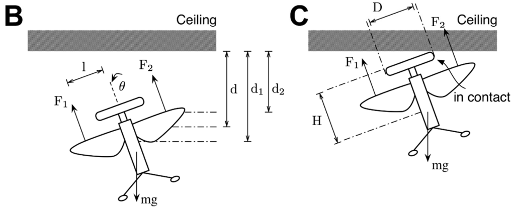
Fig. S10: Flight stability in wall proximity.
